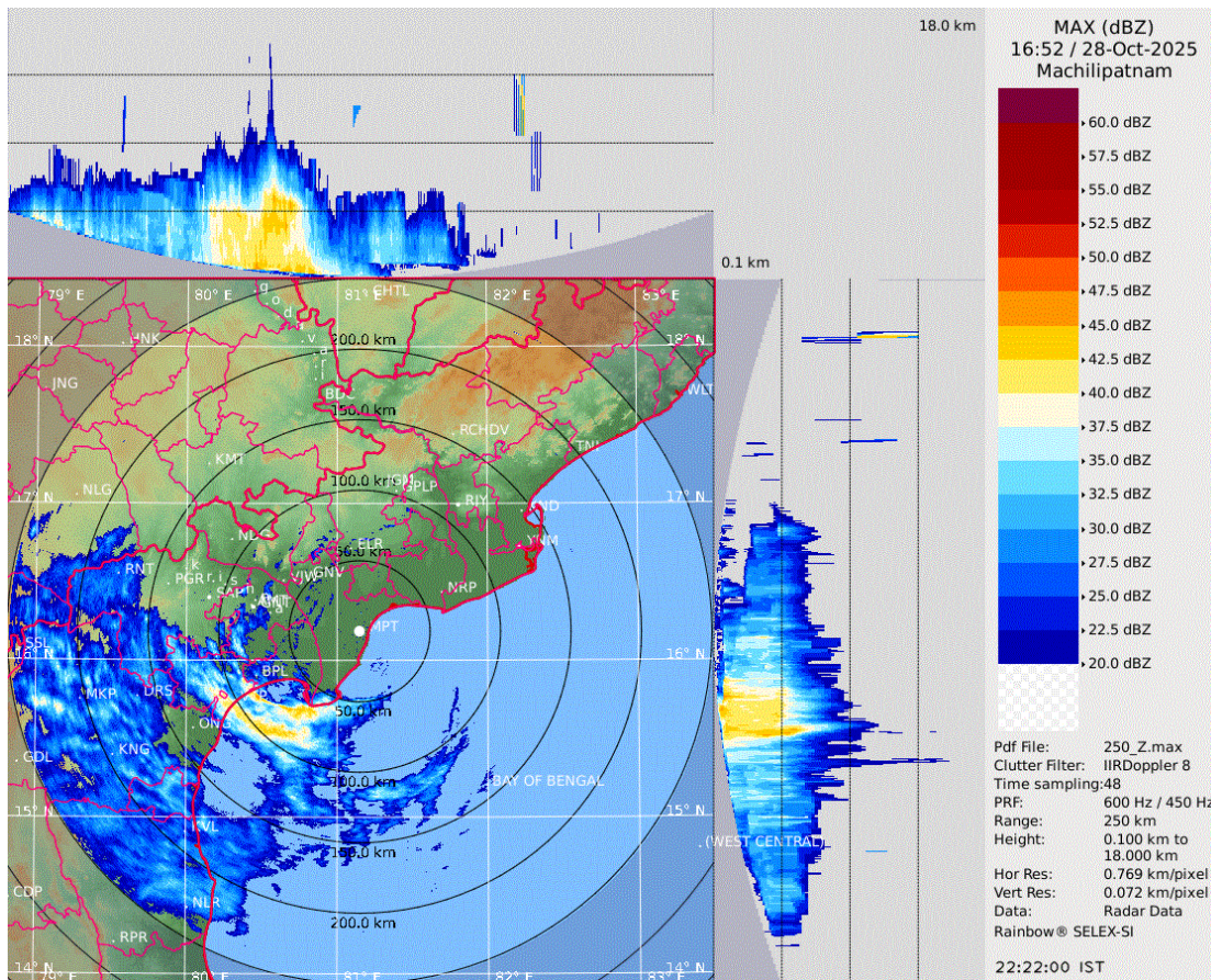
Max Z image of DWR Machilipatnam based on 1652 UTC of 28 th October 2025
