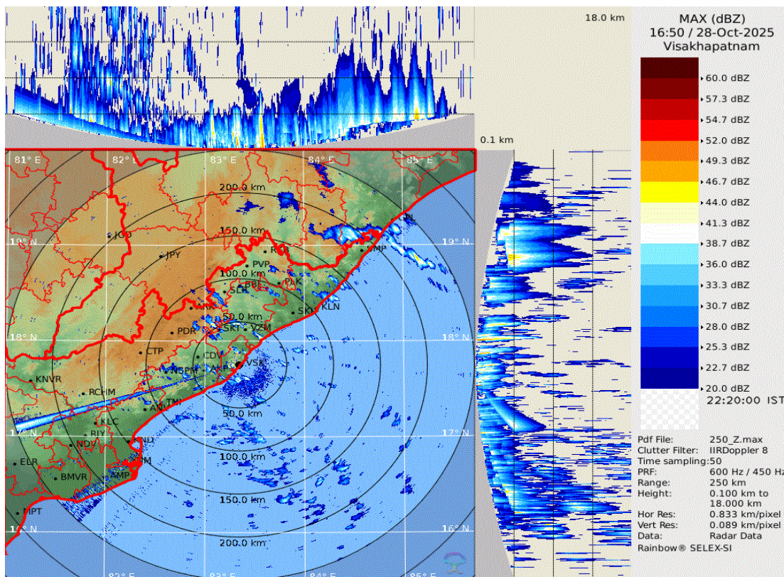
Max Z image of DWR Visakhapatnam based on 1650 UTC of 28 th October 2025
